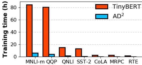
Figure 2: KD evaluation accuracy and training cost comparison when using different data augmentation schemes. TinyBERT uses text-editing based data augmentation for KD. AD 2 uses adversarial data augmentation for KD.
